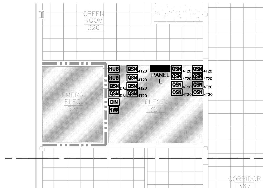
1 SECOND FLOOR — ENLARGED ELECTRICAL ROOM SCALE: 1/4" = 1'-0"
